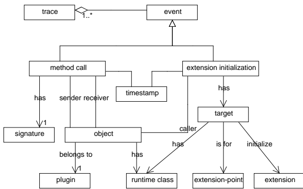
Figure 4. Trace meta model
