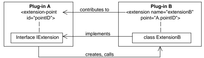
Figure 1. The Eclipse plug-in extension mechanism
