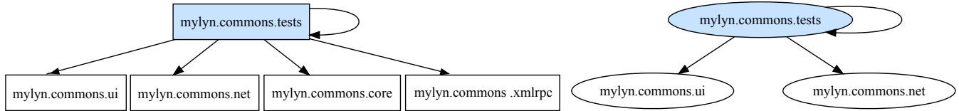
Figure 2. Static and Dynamic Dependencies of Test-Component “mylyn.commons.tests”
