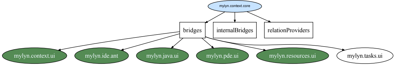
Figure 6. Static and Dynamic Dependencies based on Extension-Points: Plug-In Scope
