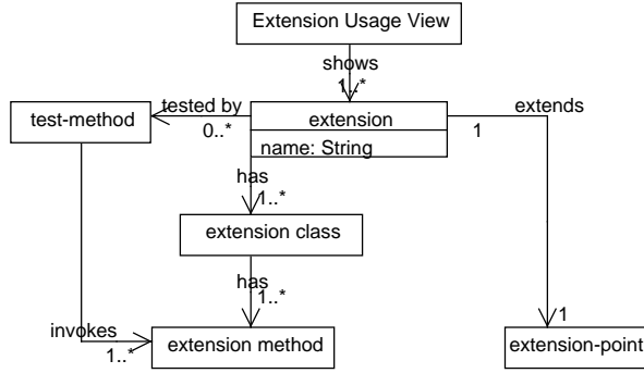
Figure 5. Meta Model: Extension Usage View
