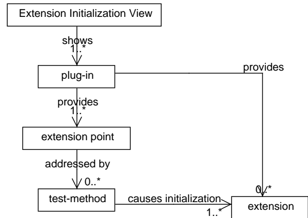
Figure 3. Meta model of the Extension Initialization View
