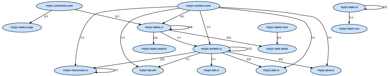
Figure 7. Static and Dynamic Dependencies based on Extension-Points: System Scope
